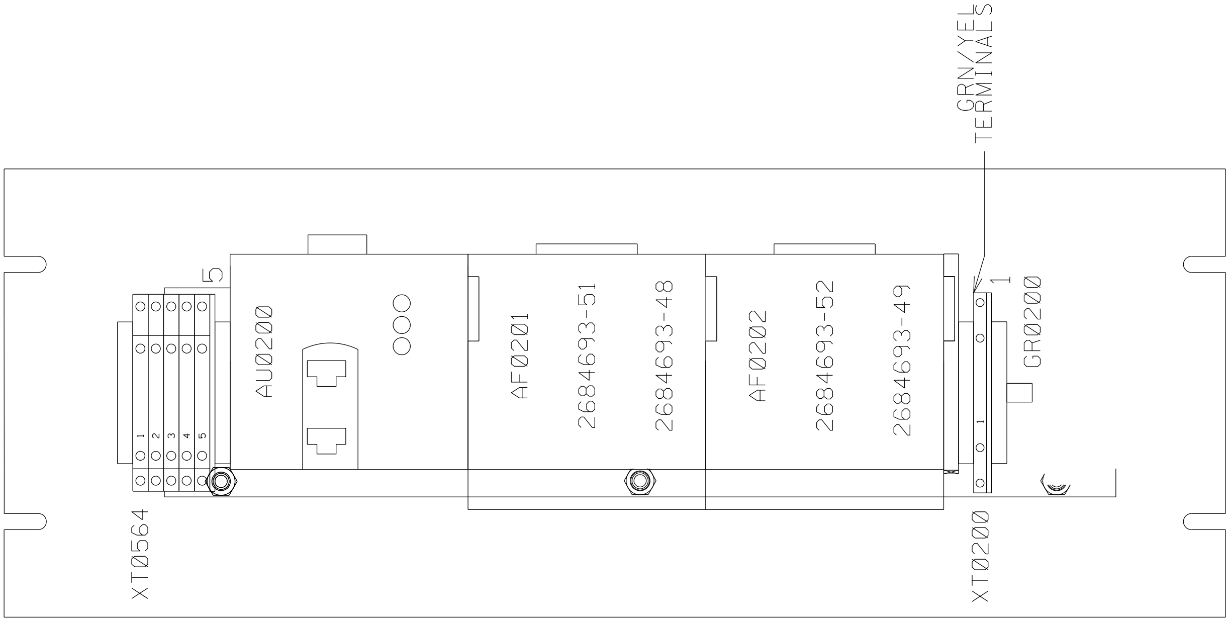
BACK VIEW WITH FLEX I/O INSTALLED
